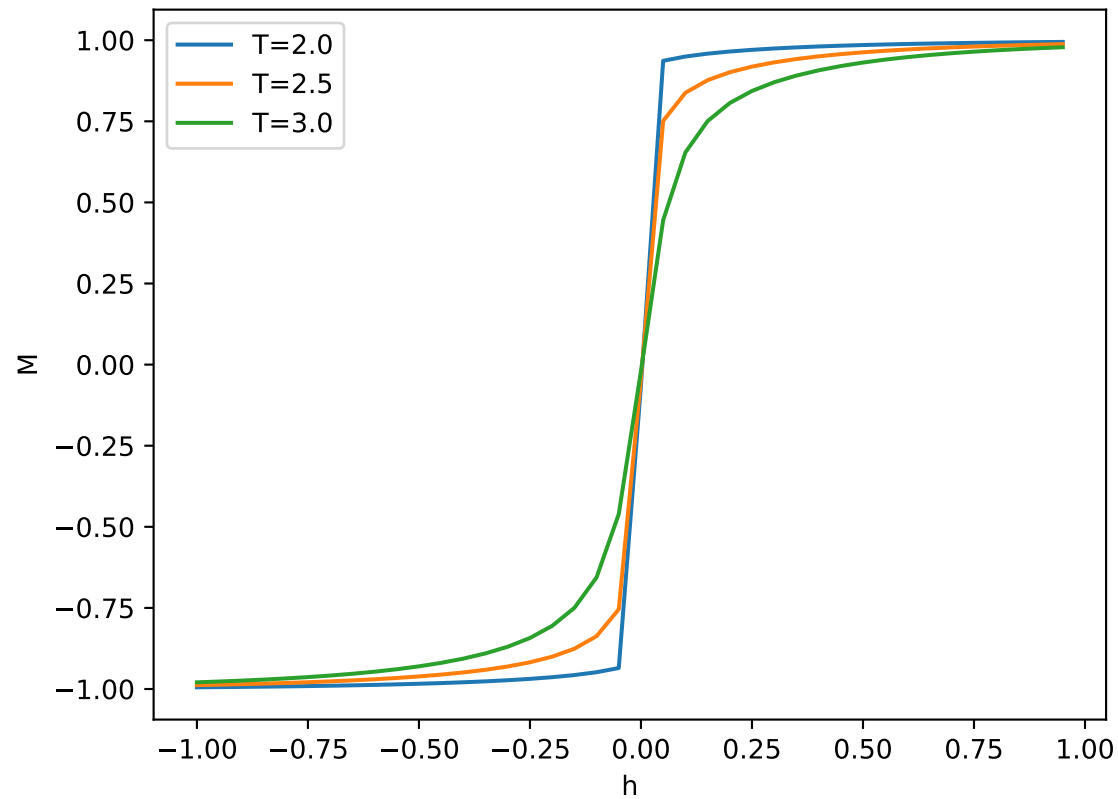
M(T,h)
